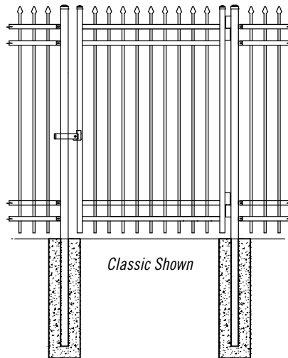
SINGLE SWING DIMENSIONAL DRAWINGS
