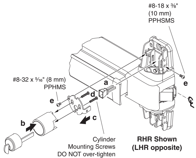
RHR Back of Device
