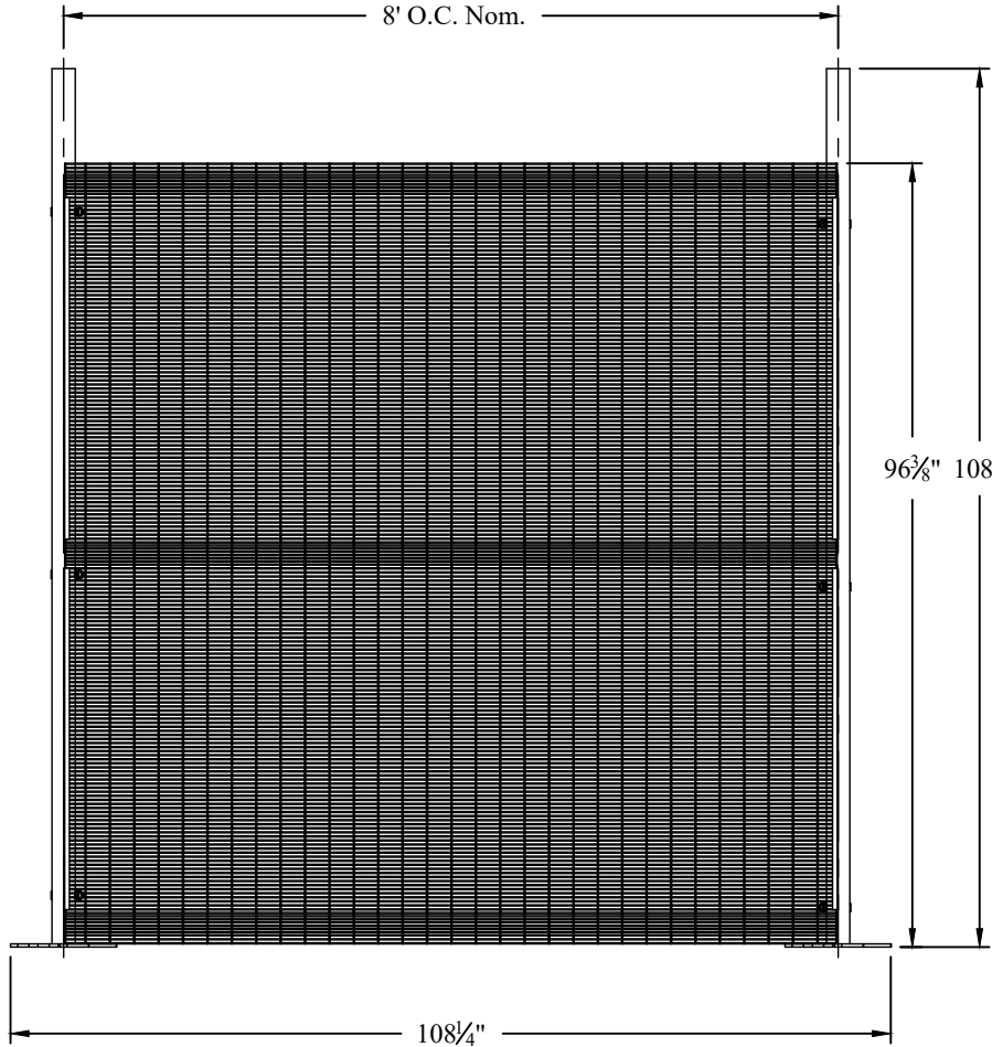
.5" x 3" x 10.5GA WIREWORKS ANTI-CLIMB MESH W/ 3 V-FOLD RIBS
