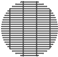
.5" x 3" x 10.5GA WIREWORKS ANTI-CLIMB MESH W/ 3 V-FOLD RIBS
