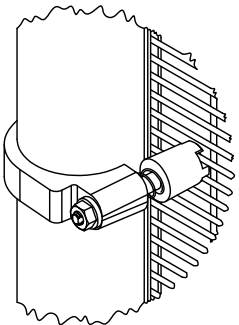
BRACKET DETAIL FROM STRUCTURE SIDE
